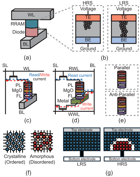
Fig. 10. RRAM and MRAM and PCRAM structures and two states for programming 0/1. (a) RRAM. (b) RRAM state. (c) STT-MRAM. (d) SOT-MRAM. (e) MRAM state. (f) Chalcogenide state. (g) PCRAM state.
