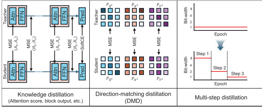
Fig. 6. Development direction of binarized (or ternarized) Transformers from leveraging knowledge distillation to multistep distillation.
