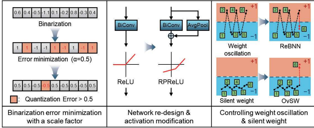
Fig. 3. Development direction of BNNs from introducing a scale factor to controlling the training quality.
