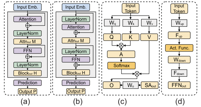
Fig. 5. Overview of Transformer architectures: BERT [15] and ViT [18] for language and vision tasks, respectively. (a) BERT. (b) ViT. (c) Attention. (d) FFN.
