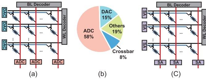
Fig. 8. Compute-in-memory architecture based on NVM. (a) nvCIM architecture. (b) nvCIM energy breakdown. (c) NVM-based BNN CIM architecture.
