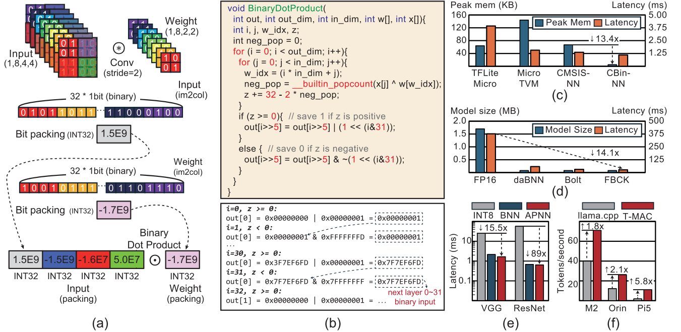
Fig. 7. (a) Overview of binary convolution with bit packing. (b) Code snippet implementing the binary dot product. (c) Comparison of peak memory and latency on an MCU, i.e., NUCLEO-144 board. (d) Comparison of model size and latency on a Raspberry Pi 3. (e) Latency comparison of cutlass-int8-TC, cutlass-BNN-TC, and APNN-w1a2 for various models on an RTX 3090 GPU. (f) Performance comparison (in tokens/s) between two libraries running a 1.58-bit LLM (BitNet-3B).
