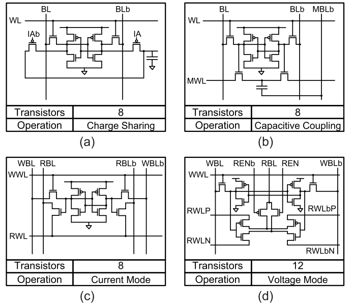
Fig. 9. SRAM-CIMbit-cell schematics. (a) Valavi et al.'s [122] charge-sharing-based 8T1C SRAM-CIM. (b) Jiang et al.'s [42] capacitive coupling-based 8T1C SRAM-CIM. (c) Oh et al.'s [12] current mode 8T SRAM-CIM. (d) Yin et al.'s [44] voltage mode 12T SRAM-CIM.
