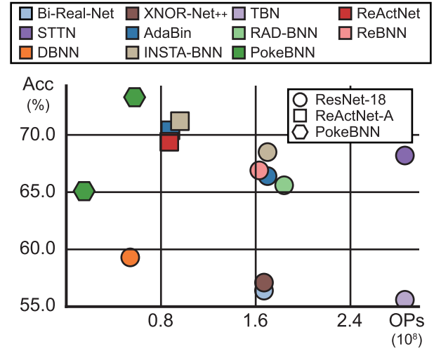
Fig. 4. Comparison of various BNN/TNN models (dataset: ImageNet-1K).
