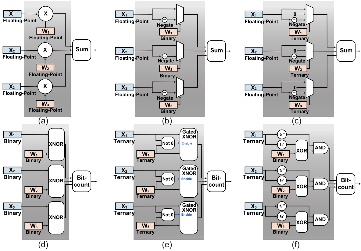
Fig. 2. Overview of the hardware realization of a dot product in (a) conventional DNNs, (b) BWNs, (c) TWNs, (d) BNNs, (e) TNNs, and (f) TBNs.
